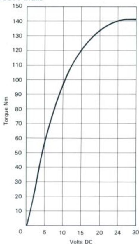
Typical Torque/voltage Characteristic PB800 Brake
